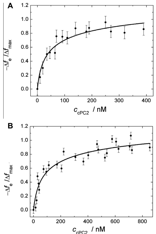
Fig. 4. Adsorption isotherms of (A) cPC2wt ( \Delta f_{\text{max}} = (18 \pm 1) Hz) and (B) cPC2S812D ( \Delta f_{\text{max}} = (23 \pm 1) Hz) interacting with PIGE14. The parameters of Eq. (3) were fit to the data.
