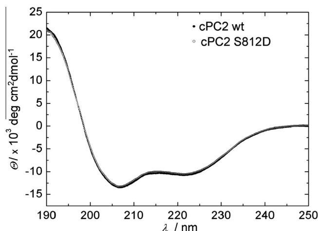
Fig. 2. CD spectra of cPC2wt and cPC2S812D mutant.
