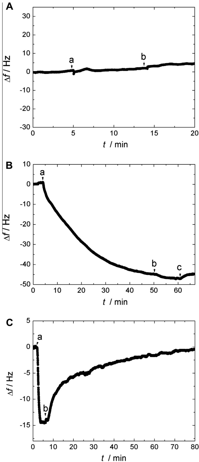
Fig. 3. Time courses of the frequency shifts after addition of: (A) (a) 0.3 \mu\text{M} PIGE14 to a DOPC–SSM and (b) rinse with buffer-B. (B) (a) 0.65 \mu\text{M} and (b) 0.73 \mu\text{M} PIGE14 to a DOPC/DOGS–NTA–Ni (9:1)–SSM; (c) indicates the time point of rinsing with buffer-B. (C) (a) 0.27 \mu\text{M} cPC2wt to a DOPC/DOGS–NTA–Ni (9:1)–SSM with bound PIGE14; (b) indicates the time point of buffer rinsing (150 mM NaCl, 20 mM \text{KH}_2\text{PO}_4/\text{K}_2\text{HPO}_4 , 1 mM EDTA, pH 7.4).
